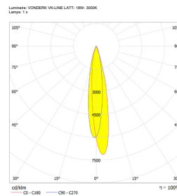
VK-LINE LATT- 18W-3000K-AL
